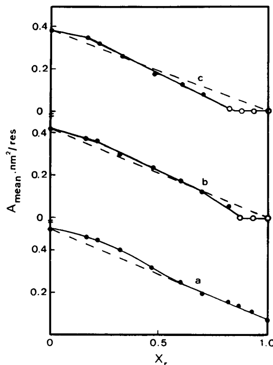
FIGURE 4 Mean area per "residue" in SP-C/DPPC films as a function of their initial composition at different surface pressures: 25 mN·m -1 (a), 50 mN·m -1 (b), 55 mN·m -1 (c). Full circles represent average results of at least two experiments. Open circles represent extrapolated values of A_{\text{mean}} at the given surface pressure.
