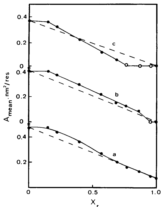
FIGURE 7 Mean area per "residue" versus monolayer composition for SP-C/DPPG mixtures at surface pressure of 25 mN·m -1 ( a ), 50 mN·m -1 ( b ), 55 mN·m -1 ( c ).
